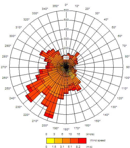
Figure 3.10.2/3 Wind rose based on 2008 data from Birmingham Airport meteorological station.
